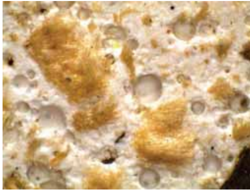
Figure 7: Cut of a MgO-board investigated in a stereo microscope at 10 times magnification.
